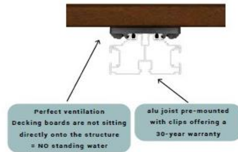
'GRAD SYSTEM' SET-UP
