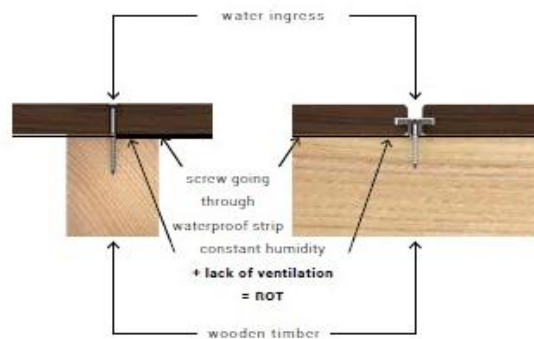
'TRADITIONAL' INSTALLATION OR WITH SIDE CLIPS
